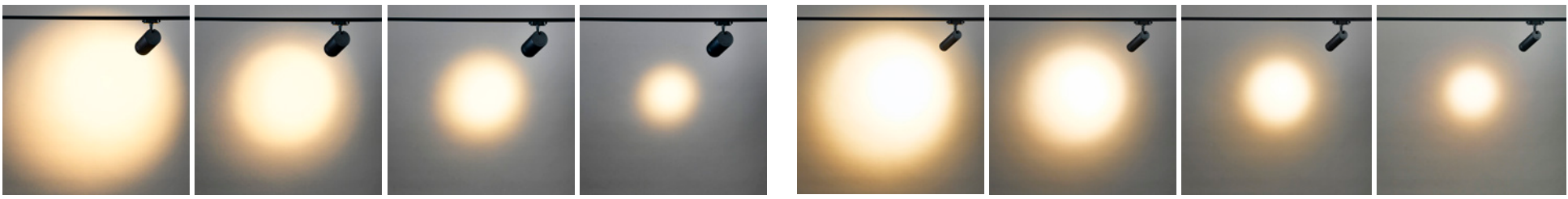
FAS_008 LAMP AC 5W, 10W LAMP AC 15W LAMP AC 20W CCT 3000K, 4000K, 5000K CCT 3000K, 4000K, 5000K CCT 3000K, 4000K, 5000K SIZE 55X115(133) / 180 SIZE 65X145 (165) / 210 SIZE 75X148 (170) / 230 BEAM ANGLE 15-60° BEAM ANGLE 15-60° BEAM ANGLE 15-60° OPTION ON/OFF, TRIAC OPTION ON/OFF, TRIAC OPTION ON/OFF, TRIAC
